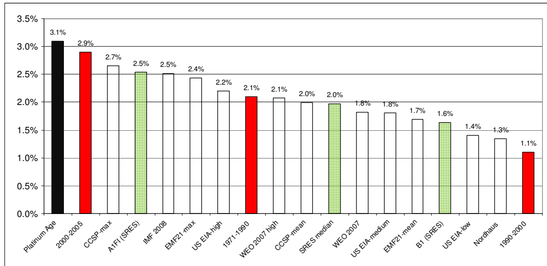
Figure 5 A comparison of annual projected growth rates in SRES and post-SRES scenarios (c. 2005-203) with historical data for global CO 2 emissions from fossil fuels and the Platinum Age projections (2005-2030).
