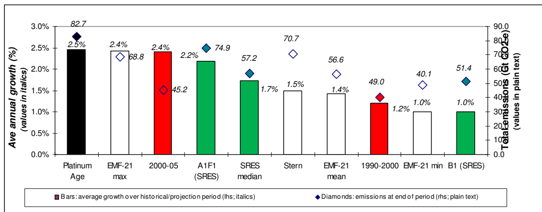
Figure 6. Comparison of Platinum Age projections with other projections and historical data in terms of average growth rates (bars; italics; left axis) and total emissions (diamonds; plain text; right axis)
