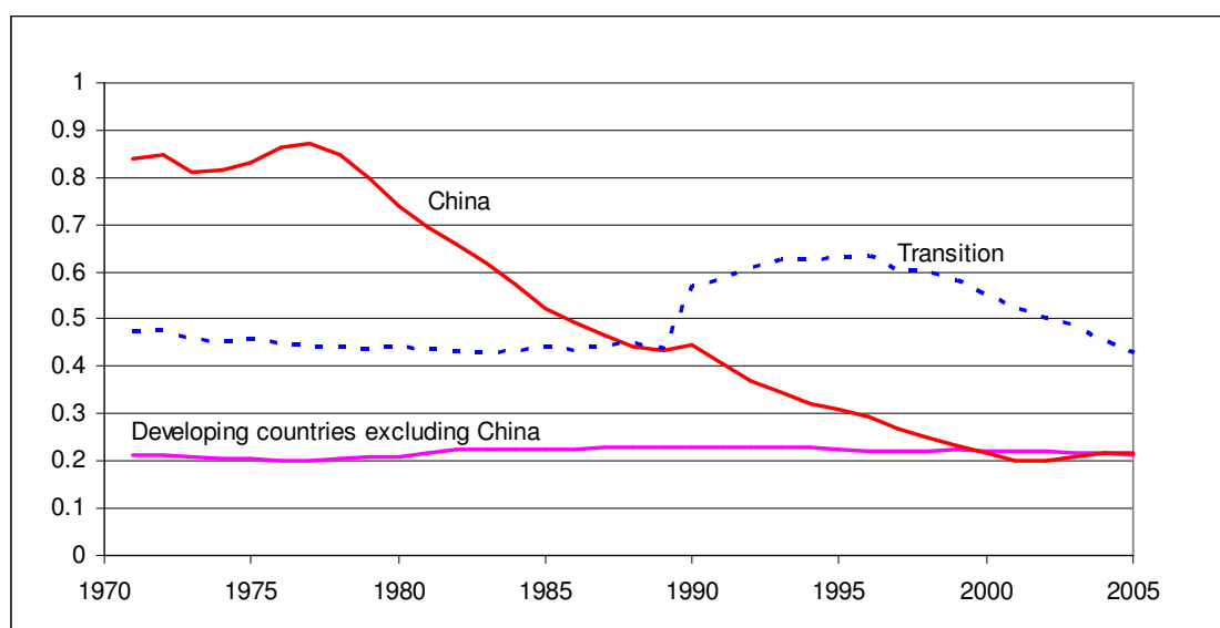
Figure 2 Energy intensities of GDP for China, other developing countries, and transition countries, 1971-2005.
