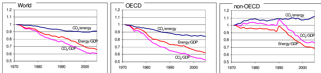
Figure 1 Emissions/GDP, Energy/GDP and Emissions/Energy for the world, OECD and non-OECD, 1971-2005 (1971=100)
