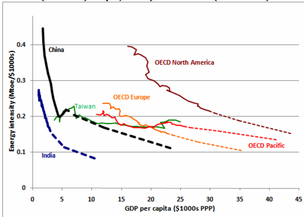
Figure 4 Energy intensity and GDP per capita for various countries and regions: historical (solid lines) and projected by the 2007 WEO (dashed lines)
